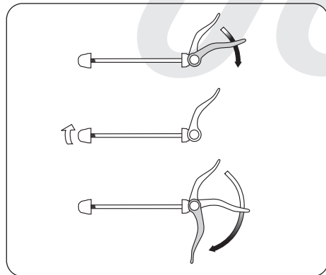
Instelbout vergrendelen
