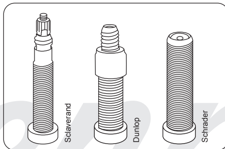
Types de valves
