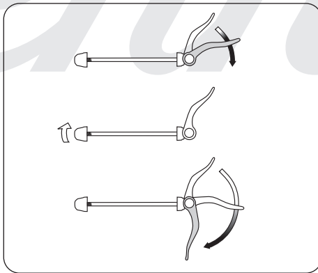
Instelbout vergrendelen
